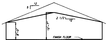
SECOND FLOOR ELEVATION SECTION B - B N.T.S.
