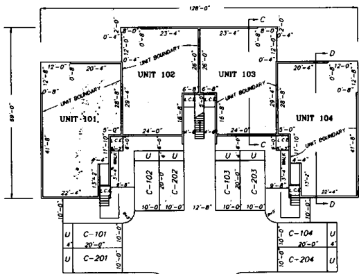
FIRST FLOOR PLAN BUILDINGS 11, 12, 13 & 14 SCALE 1" = 20'
