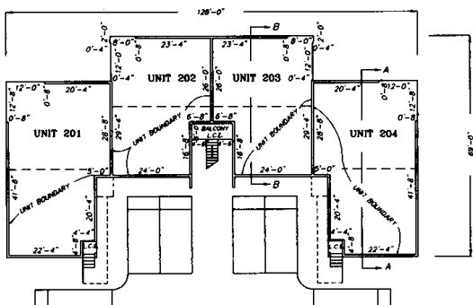
SECOND FLOOR PLAN BUILDINGS 11, 12, 13, & 14 SCALE 1" = 20'
